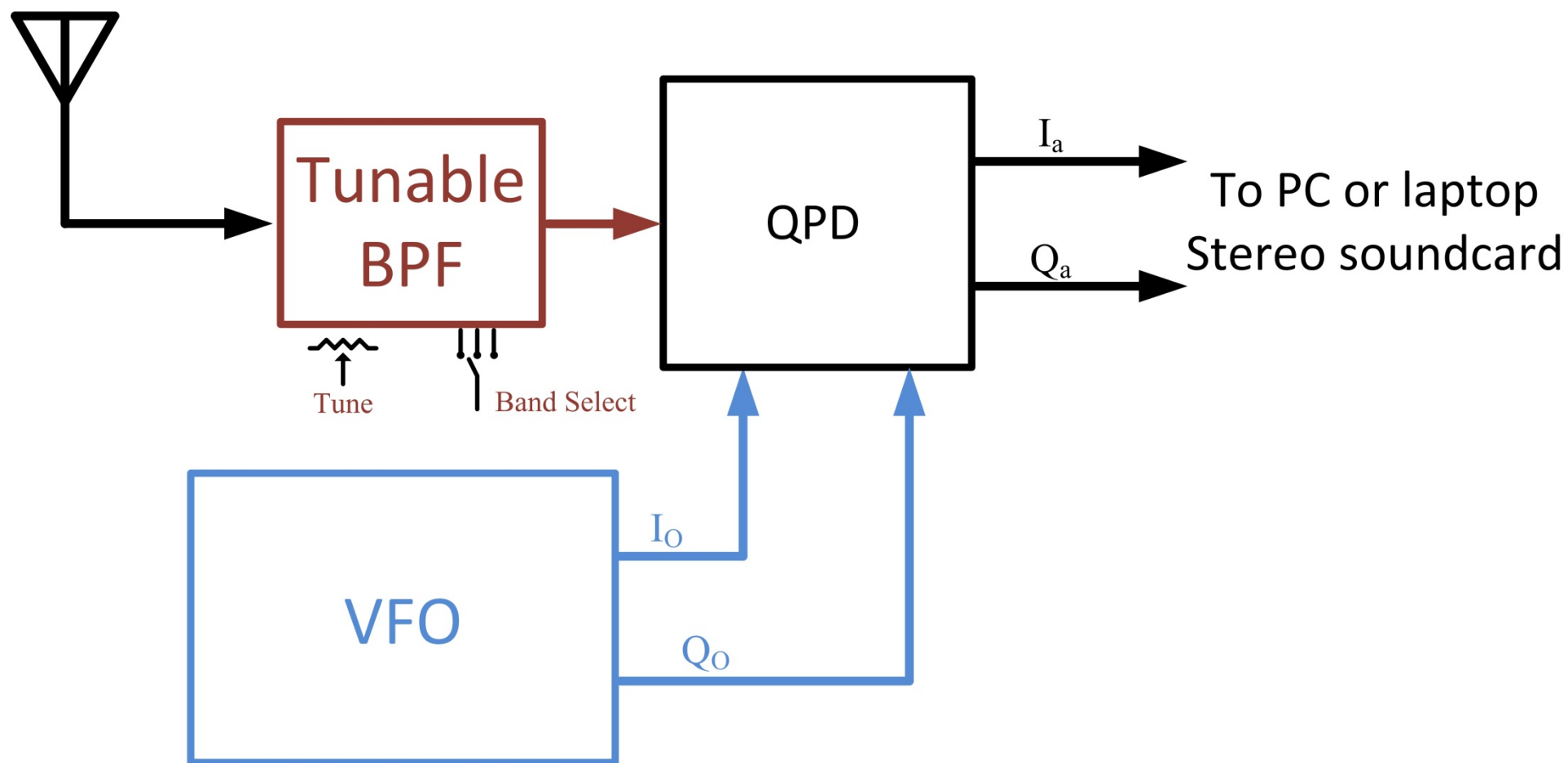
Figure 1. Basic block diagram
