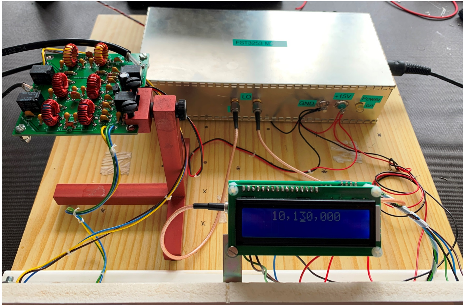
Figure 2. The three modules connected.
