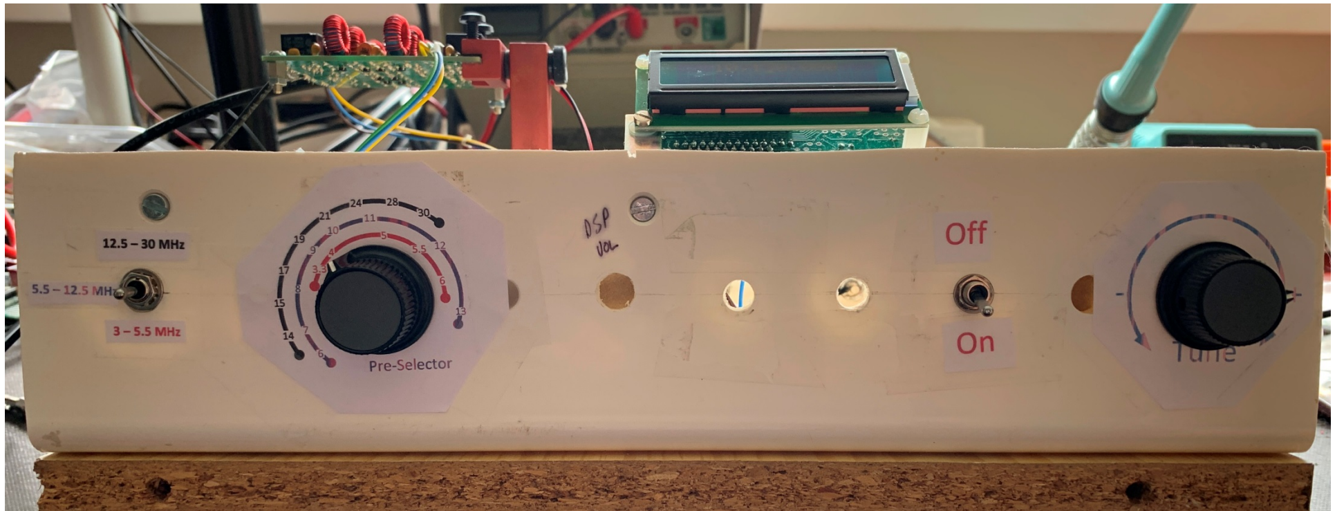
Figure 4. A view of the front panel
