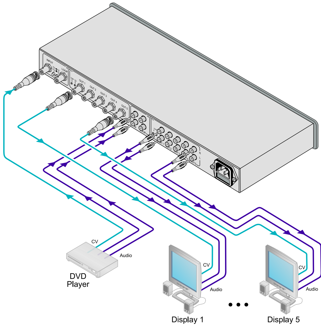
Figure 5: Connecting the VM-5AII
