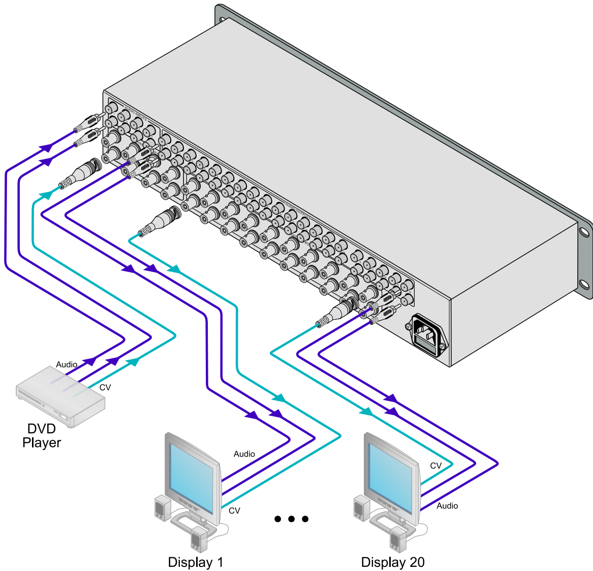
Figure 6: Connecting the VM-20ARII
