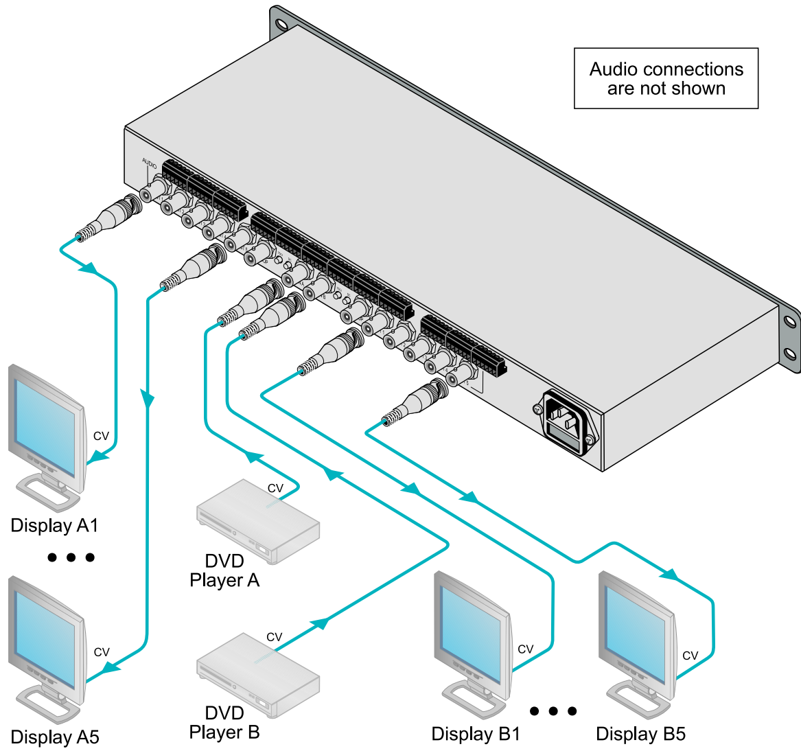
Figure 7: Connecting the VM-1411
