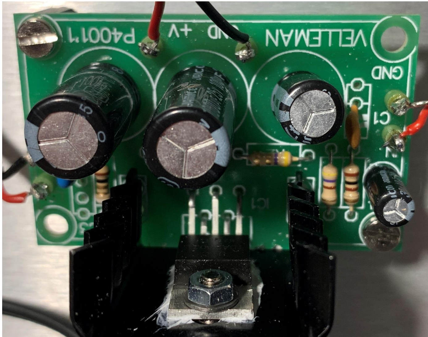
Figure 3. Power Amplifier module
