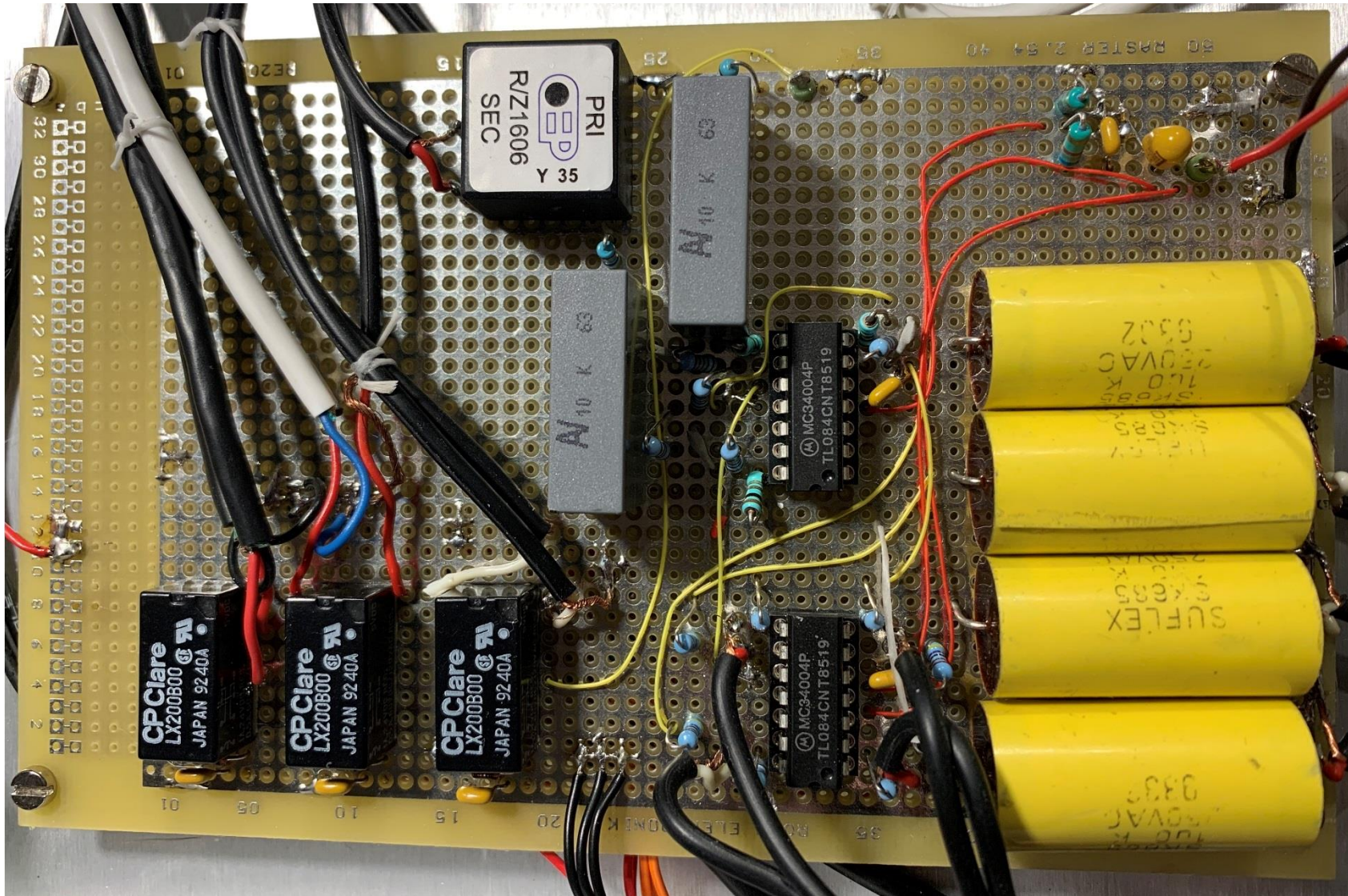
Figure 1. Hardwired Mixer Board
