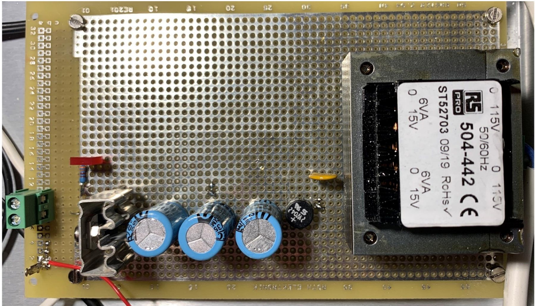
Figure 4. Power supply
